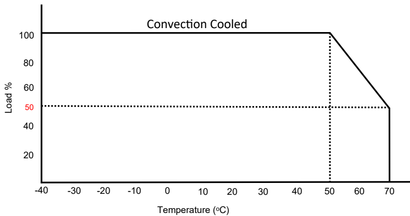
Derating curve
